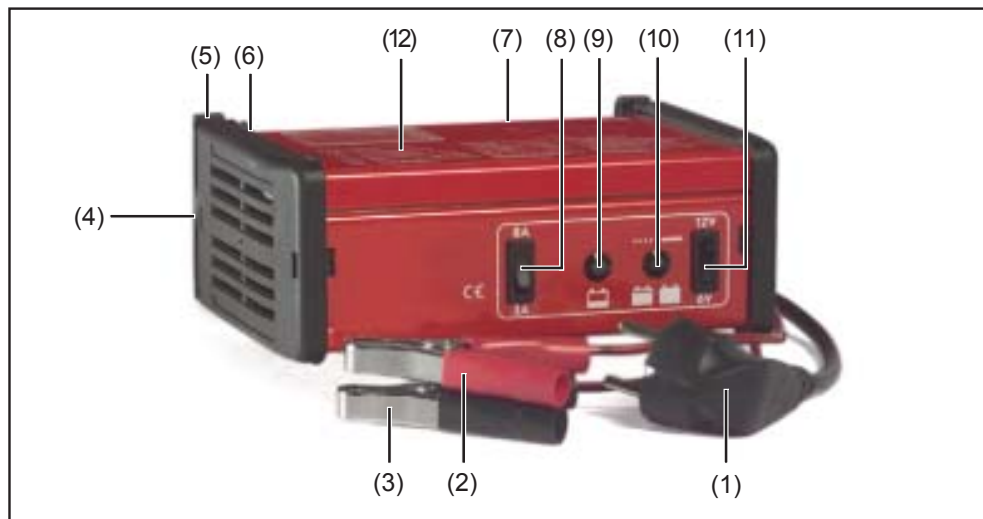
Fig. 1 Controls and connections
