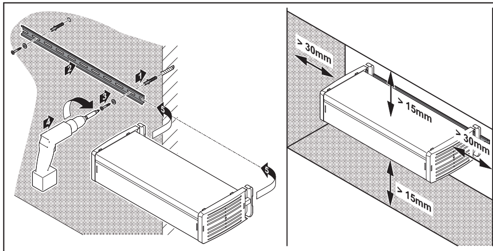
Fig. 2 Charger with optional wall bracket (DIN rail TS 35, EN 50022) Fig. 3 Minimum clearances
